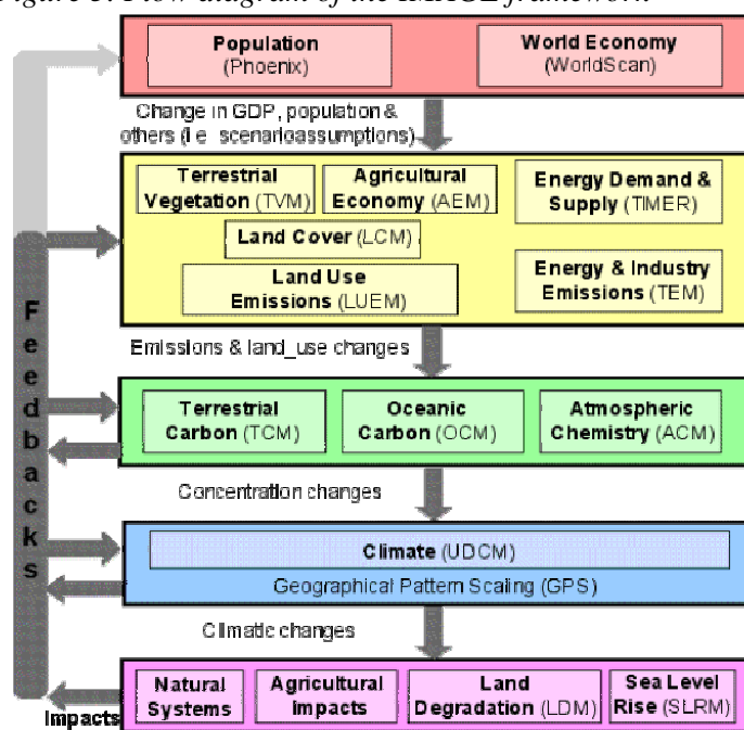
Figure 3. Flow diagram of the IMAGE framework
